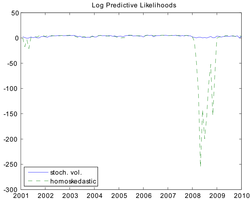
Figure 2: Log predictive likelihoods for models with Lasso prior on constant and time-varying coefficients, h = 12
